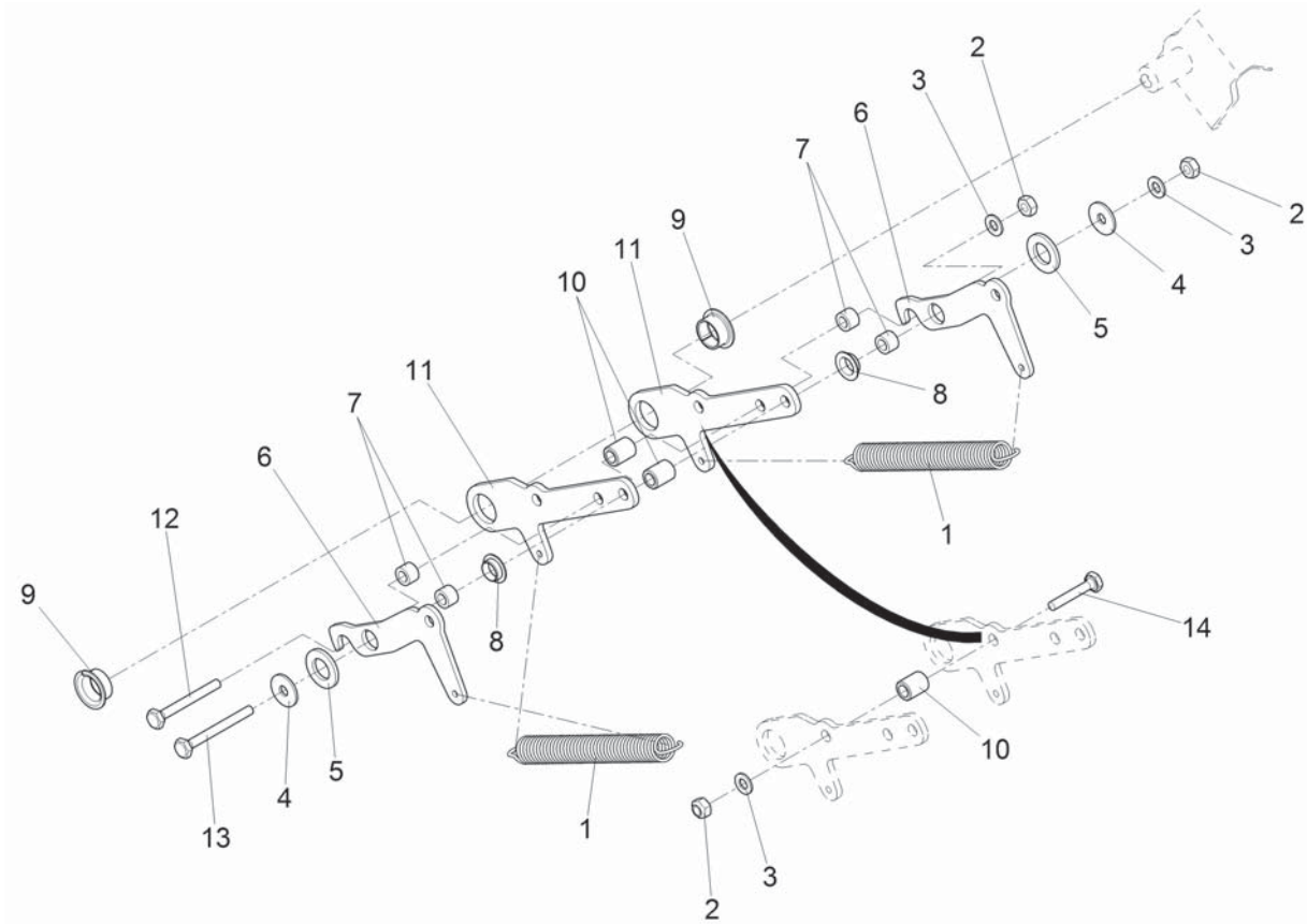
PARTS LIST - LEVER ASSEMBLY
