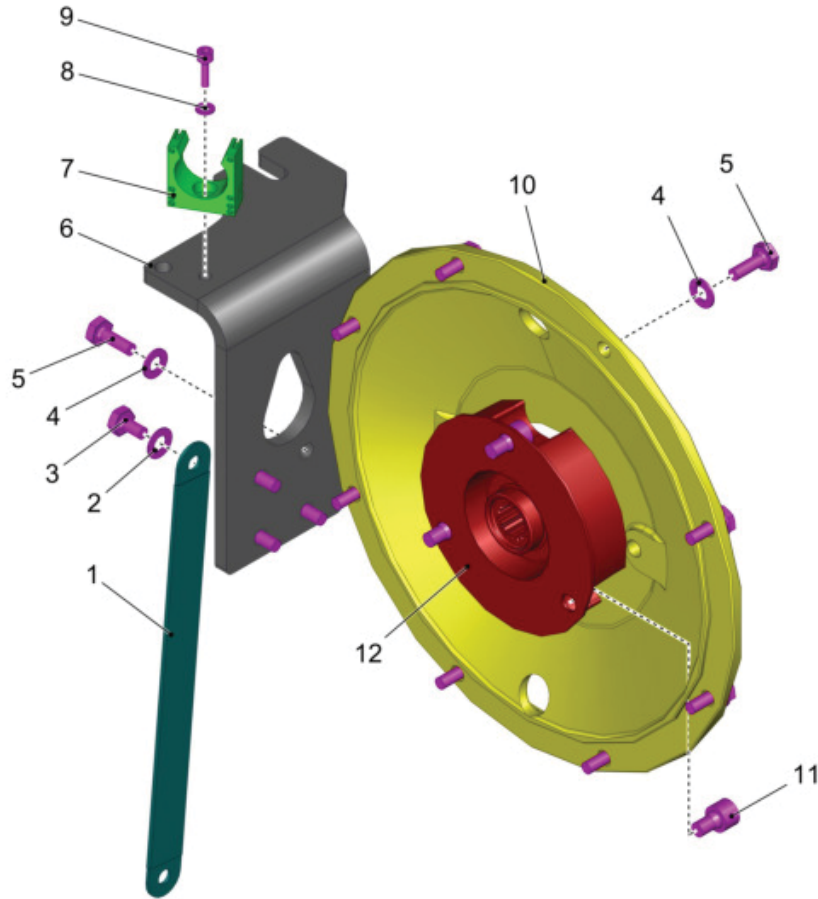
PARTS LIST - MOTOR GROUP
