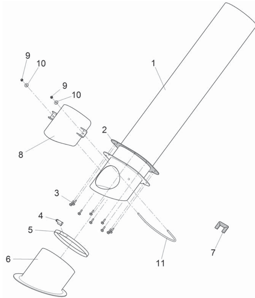
PARTS LIST - SUCTION PIPE ASSEMBLY
